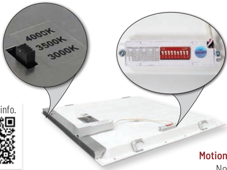
Frame Light
