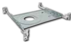
Universal New Construction Frame-In for 4" Downlight only NF-R246
