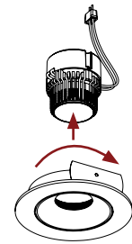
Attach LED module/driver and thread clockwise
