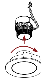
Attach LED module/driver and thread clockwise
