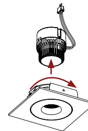
Attach LED module/driver and thread clockwise
