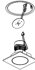
Connect MR16 GU5.3 adapter
