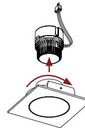
Attach LED module/driver and thread clockwise
