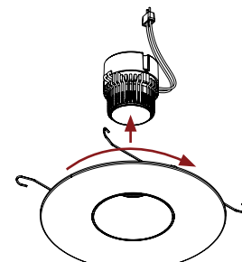
Attach LED module/driver and thread clockwise
