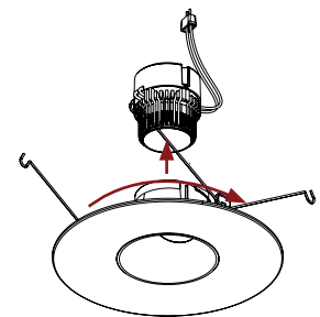
Attach LED module/driver and thread clockwise
