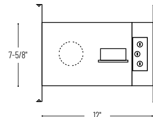
3-1/4" Ceiling Cut-Out
