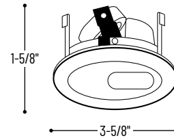
NL-3345N Natural Metal Ring
