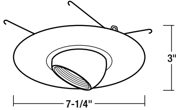
Trim OD: 7-1/4" Height: 3"
