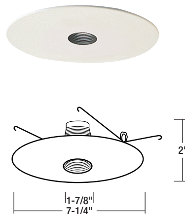
Trim OD: 7-1/4" Aperture: 1-7/8" Height: 2"
