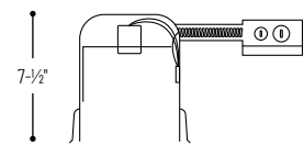
6-3/8" Ceiling Cut-Out
