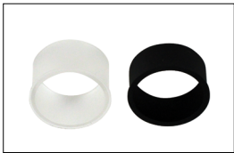
Opaque Collar Snoot NIO-AS14(color) 5/8" length NIO-AS19(color) 3/4" length NIO-AS26(color) 1" length Color: BLK Black, MPW Matte Powder White, WH White
