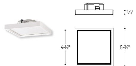
NLOS-S42L 4" Square SURF
