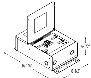
NMT-303/24C2D1 / NMT-303/24C2D2 24V Class II Dimmable Hardwire Magnetic LED Driver
