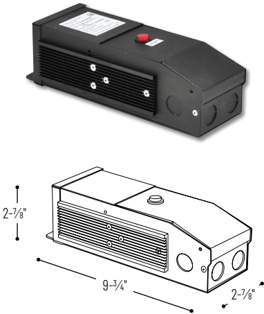
NMTD-60/24D / NMTD-96/24D 24V Class II Dimmable Hardwire Magnetic LED Driver
