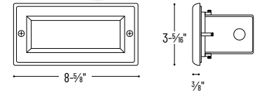
NSW-852/32 Lensed
