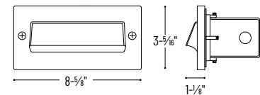
NSW-853/32 Shroud
