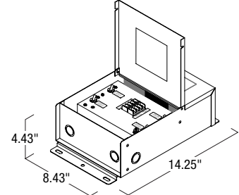
NMT-303/24C2D1: 120V/24V 300W C2 Dimm. Driver NMT-303/24C2D2: 277V/24V 300W C2 Dimm. Driver
