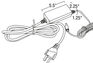
NATL-596: 24V 96W Direct Plug-In Driver
