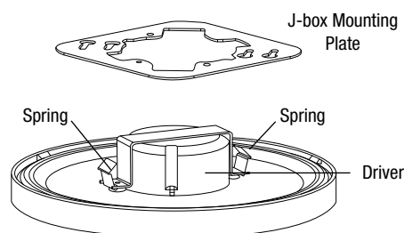
FIGURE 3 (J-box and Wires Removed for Clarity)
