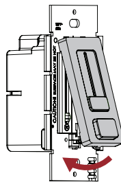
c. Insert replacement face plate into top housing groove. Position housing slider and face plate slider at minimum brightness (bottom level) and pop on face plate
