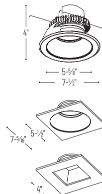
NLCBC2-656 6" Square w/ Square Aperture BB, BW, BZBZ, HZW, MPW, NN, PW, WW
