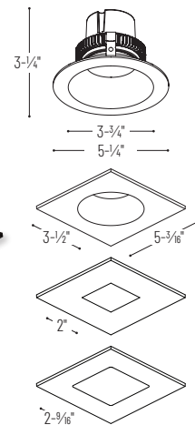
NLCBC2-456 4" Square w/Square Aperture BB, BW, BZBZ, HZW, MPW, NN, PW, WW
