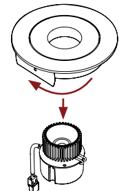
Attach LED module/driver and thread clockwise
