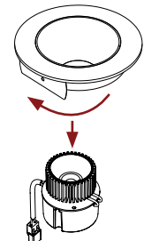
Attach LED module/driver and thread clockwise
