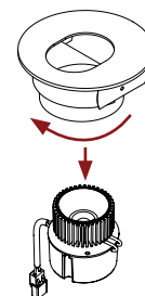
Attach LED module/driver and thread clockwise
