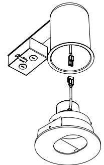
Connect luminaire and install
