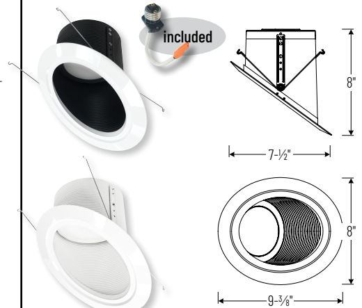
NLRS-6S11 Super Sloped Reflector
