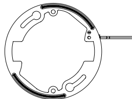
(1) 4" Mounting Bracket
