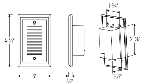
NSW-644 Vertical Louver
