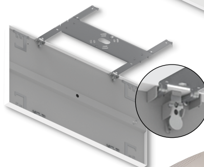
Hinged Bracket for easy installation in various ceiling types
