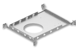
New Construction Frame-In with Collar
